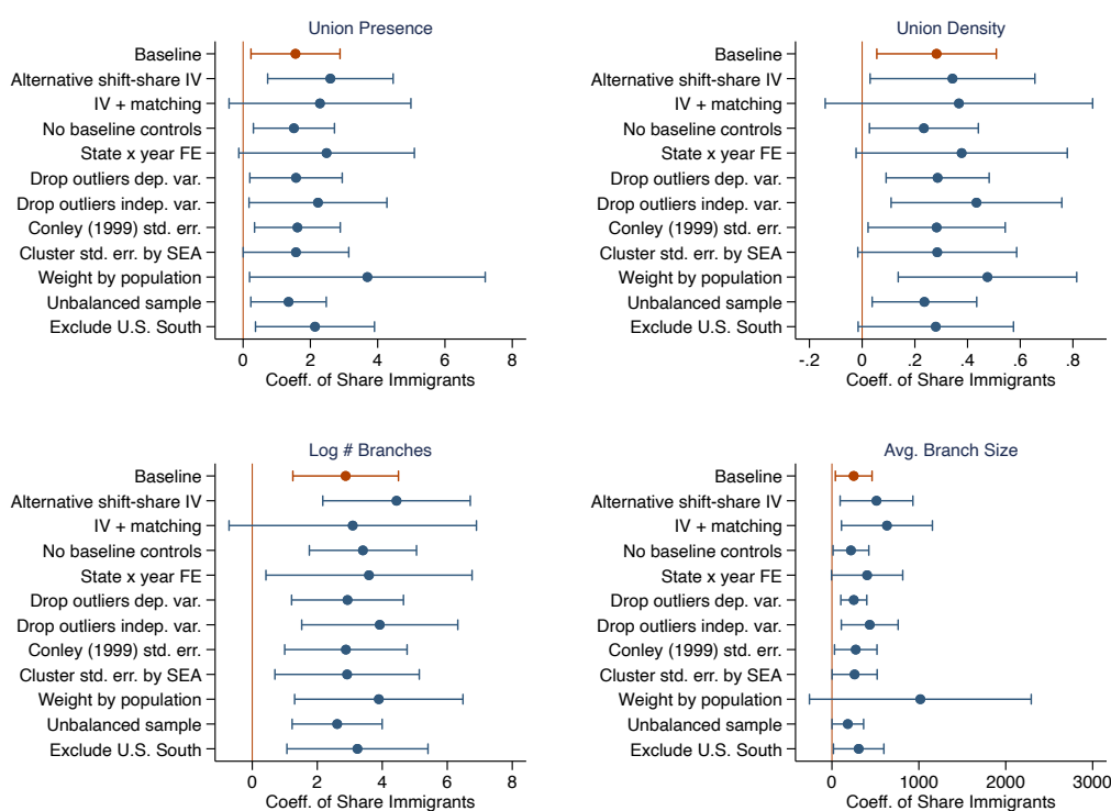
Figure 7: Summary of Robustness Checks
